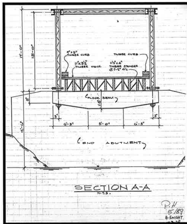
NYSDOT Inspection sketch 1978 and repeated in 1989 Inspection
