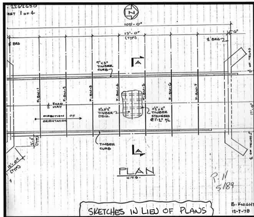
NYSDOT Inspection sketch 1978 and repeated in 1989 Inspection
