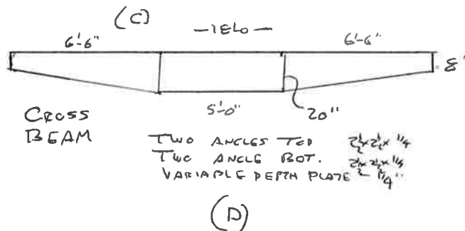
Detail Sketches of built up members
